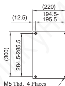
Mountain Hole Dimensions
