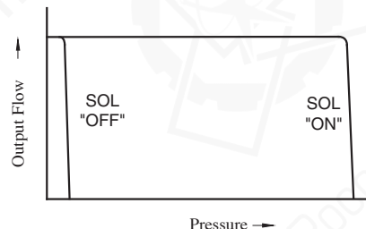
Performance Characteristics
