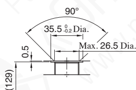
Detail of Drain Port \star 4
