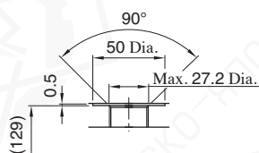
Detail of Drain Port \star 2
