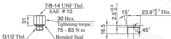
Detail of Adapter Port ★3
