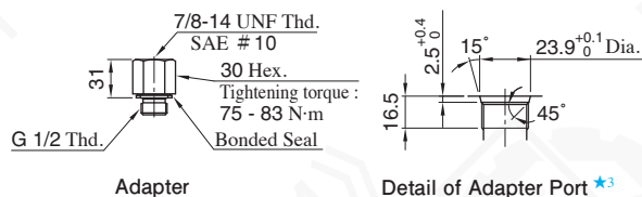
Detail of Adapter Port ★3
