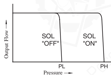
Performance Characteristics
