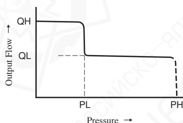
Performance Characteristics
