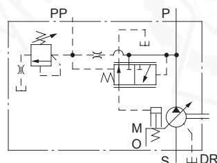
Graphic Symbol
