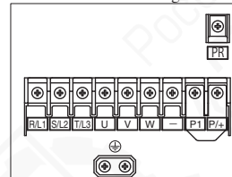
Main Circuit Terminal Assignment (B)
