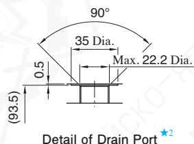
Detail of Drain Port ★2
