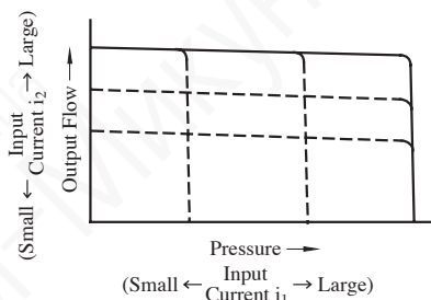
Performance Characteristics
