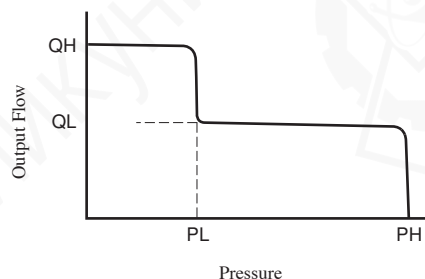
■ Performance Characteristics
