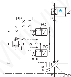
Graphic Symbol
