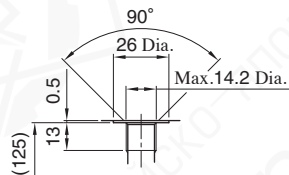
Detail of Pilot Port ★3
