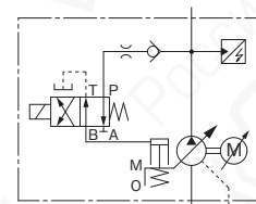
Dual Displacement Type ASE * W
