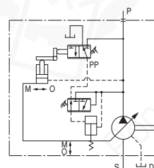
Graphic Symbol
